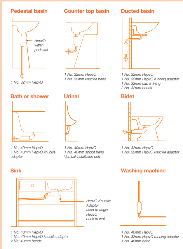
Figure 9. Hep v O mounting options
