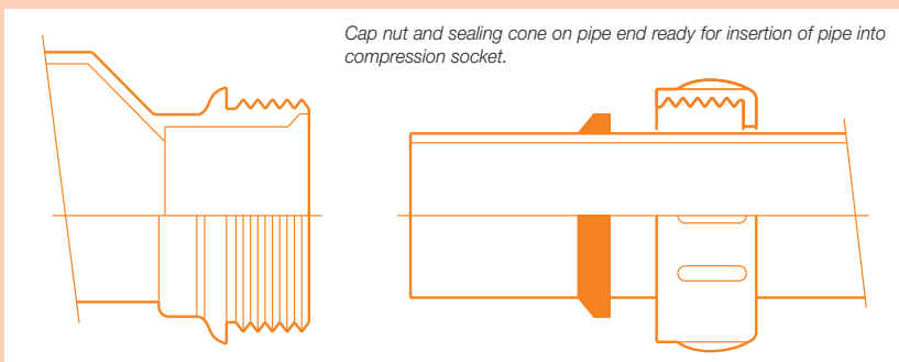
Figure 8. Hep v O outlet connection
