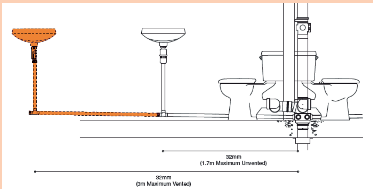
Figure 5. Schematic view for extended pipe run
