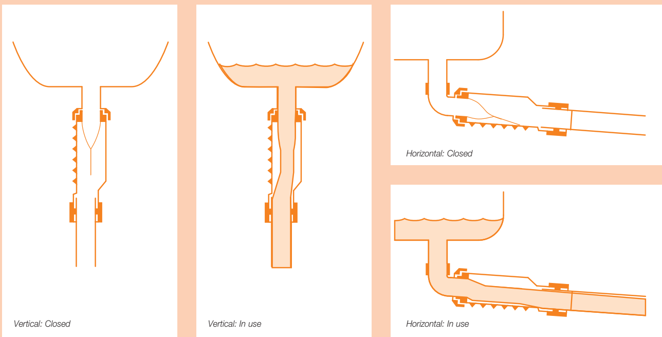
Figure 12. Operation of Hep v O
