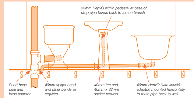
Figure 10. Hep v O installation in a typical bathroom
