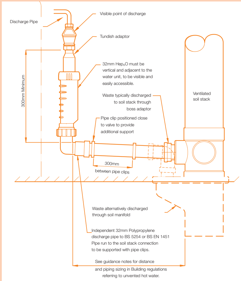
Figure 6. Self-sealing valve when used with a combined temperature and pressure relief valve for unvented hot water storage system
