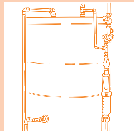
Figure 11. Tundish adaptor kit installation on an unvented hot water storage system
