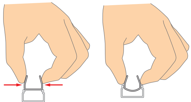
When inserting U-Clip 30 in 25x16mm trunkings, gently squeezing the upright tabs causes the base to compress for tight fitment in Size 2 trunkings.
