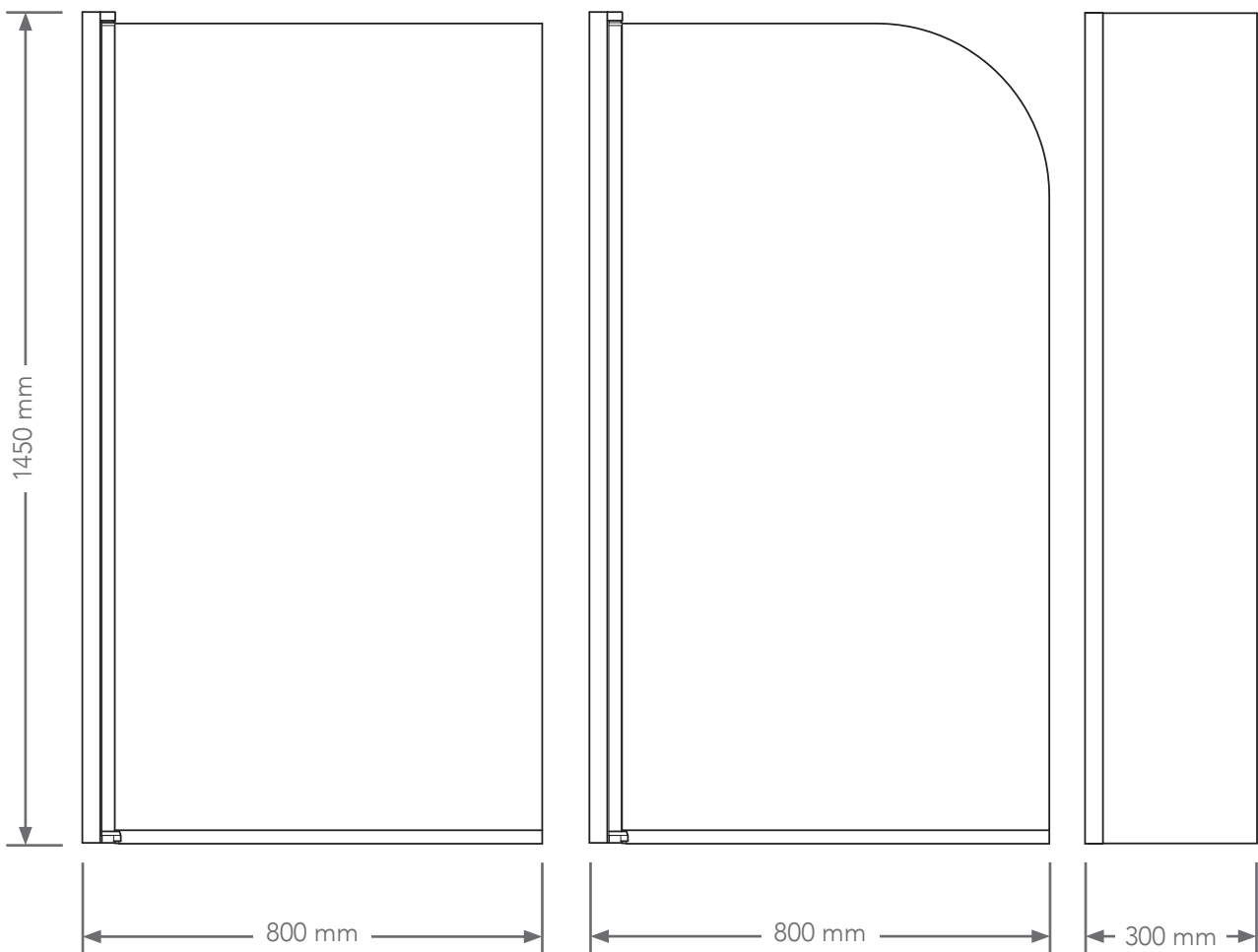
Bathscreen
