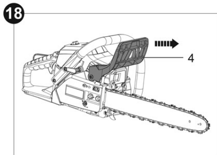
The chain brake in the engaged position, the saw chain is stopped as soon as the chain brake is activated (Fig. 18).
