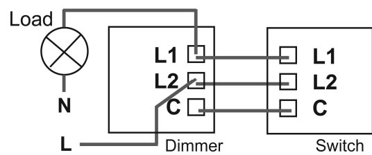
Figure 4. Using a 2-Way Dimmerswitch (For single switches or each module of a multi-gang)
