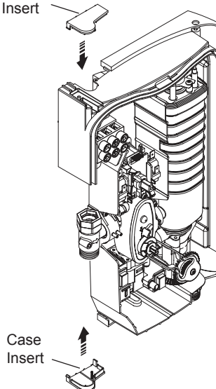
Case Insert
