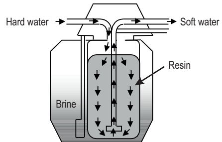
SOFTENING CYCLE
