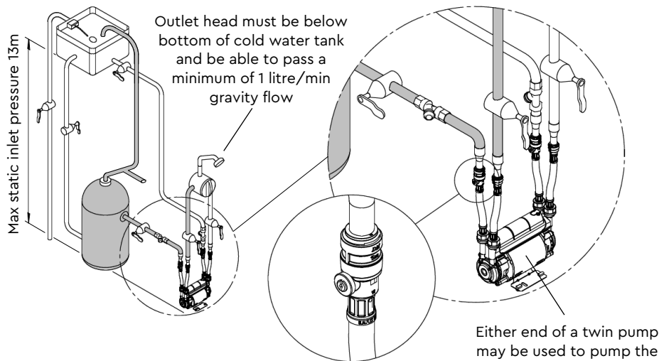
Figure 5 Standard Twin Pump System
