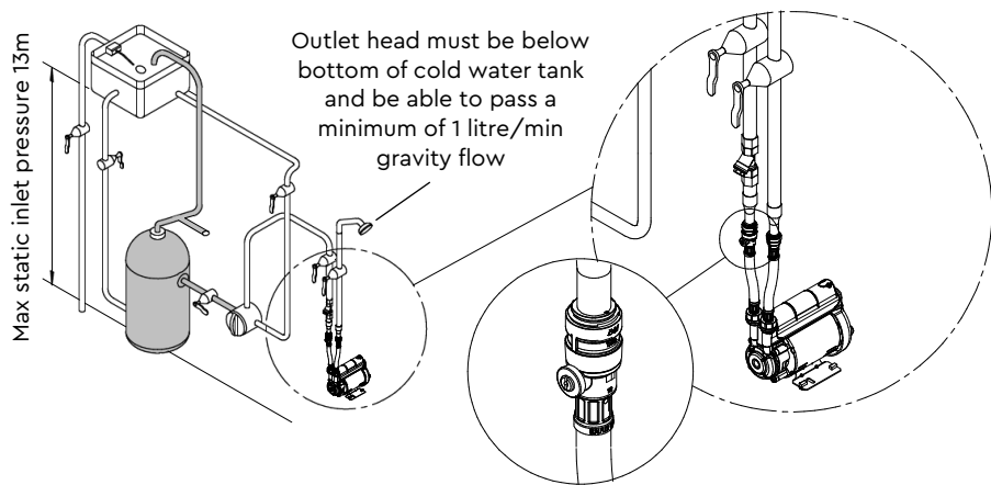
Figure 4 Standard Single Pump System
