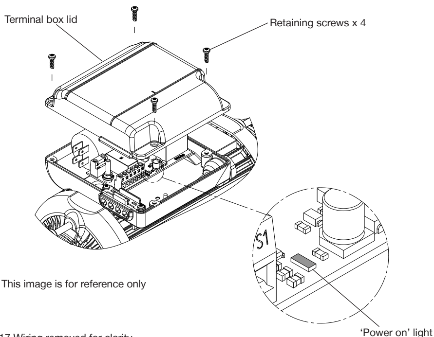
Fig. 17 Wiring removed for clarity
