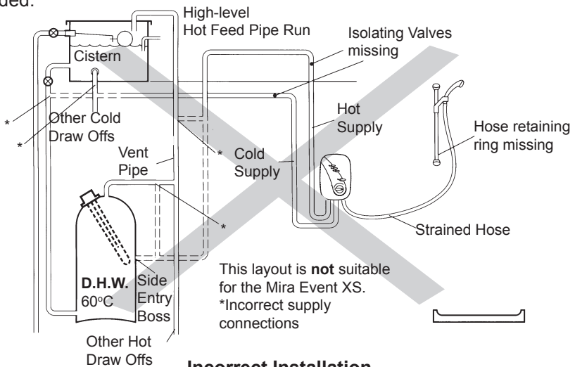
Incorrect Installation
