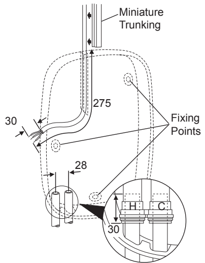
Trim the thinned section of the case covering the cable channel.
