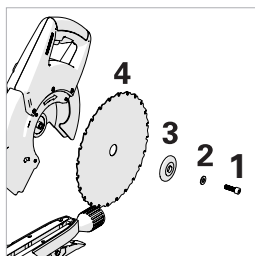
Image. 41 View of (1) Arbor screw, (2) Washer, (3) Blade flange, (4) Blade
