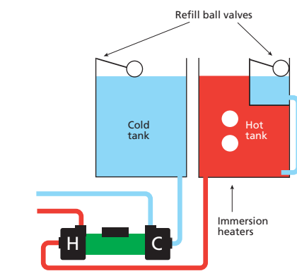
Figure 23: Elson (type) tanks
