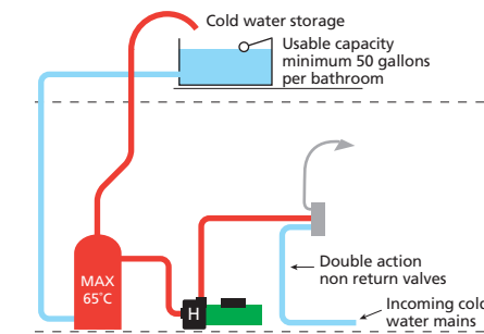
Figure 15: Tank fed (hot) with mains cold system
