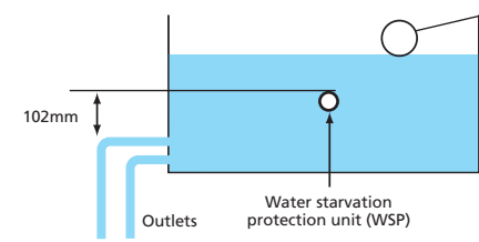
Figure 25: Water starvation protection unit (WSP)
