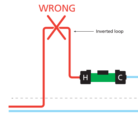
Figure 31: Inverted loops
