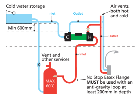
Figure 6: Right pump fitted in loft above cylinder outlet
