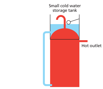
Figure 24: Fortic (type) tanks and pre-assembled units
