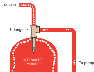
Figure 29: S flange
