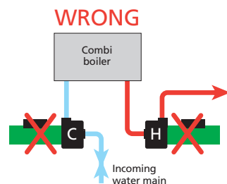
Figure 27: Combi boilers
