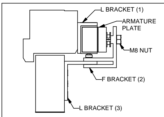
ASSEMBLED ELECTRO MAGNET
