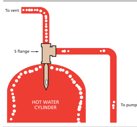
Figure 13: S flange
