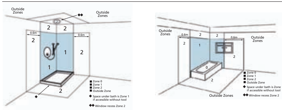
Figure 5: Bathroom Zones
