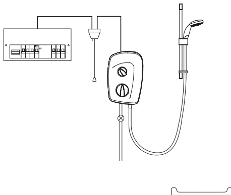
Plumbing and Electrical Schematic
