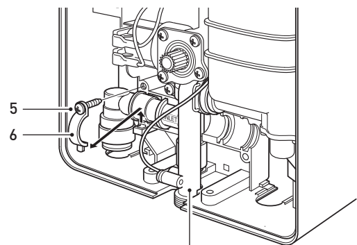
Outlet connection 7
