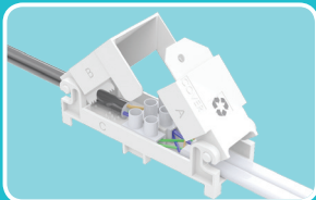
Step 4 - Close lid A & hold in position whilst closing lid B
