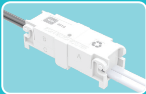
Step 5 - Clip the lid shut. Use optional screw if required
