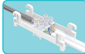
Step 2 - Place electrical connection on to base*
