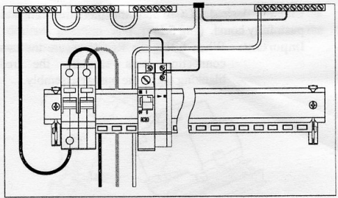
Fig 7.3 Connections to RCBOs
