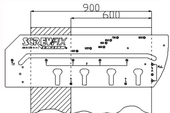
DIAGRAM C MALE JOINT - LAMINATE FACE DOWN
