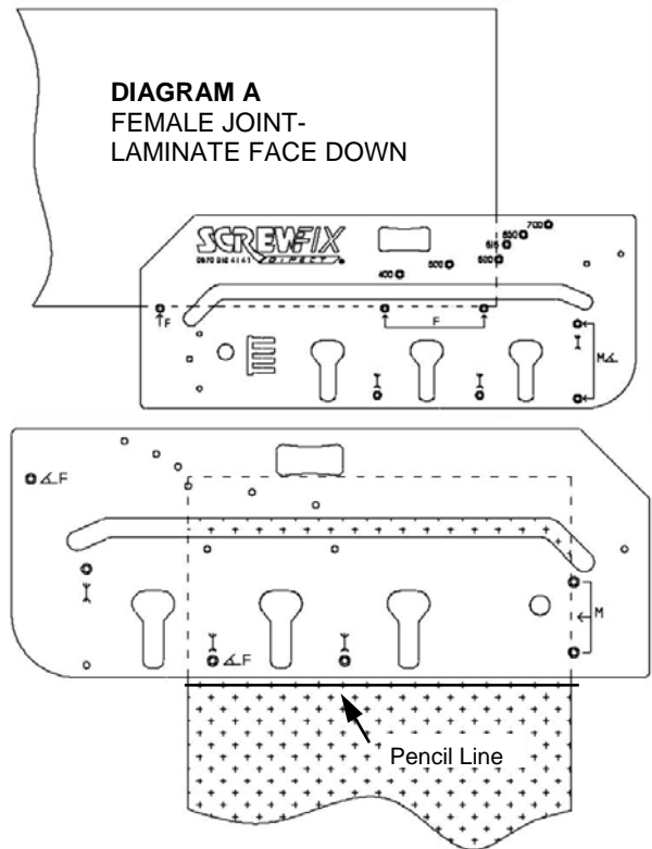
DIAGRAM B MALE JOINT- LAMINATE FACE UP
