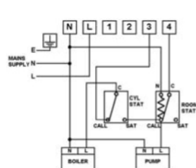
2. Gravity Hot water with Pumped Heating via RoomStat and CylinderStat
