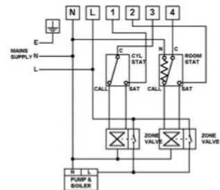
7. Fully Pumped System using RoomStat and CylinderStat and Two (2 Port) Motorised Valve with Auxiliary Switches
