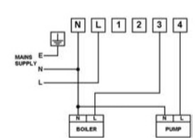
1. Gravity Hot water with Pumped Heating
